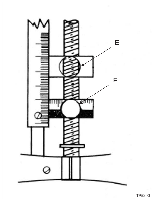
Figure 2.6 - Quill Stop Knob and Micrometer Nut
