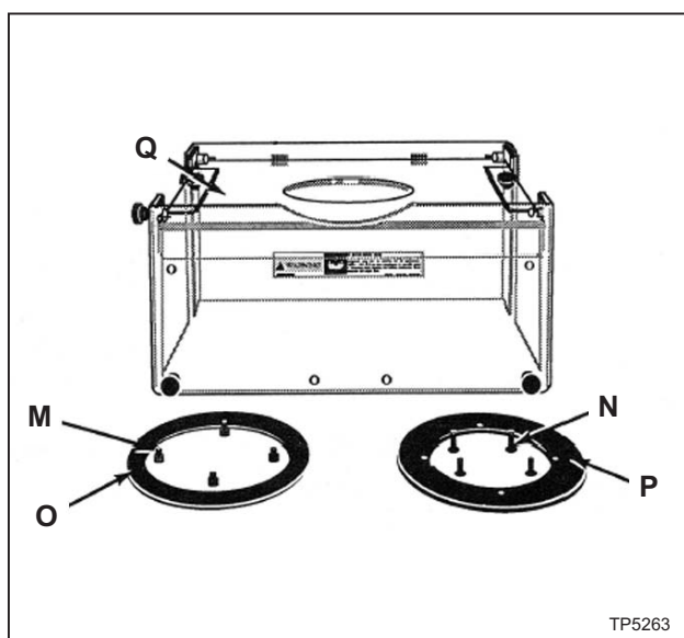
Figure I.II - Spindle Guard Assembly
